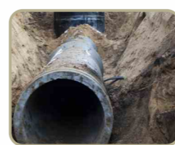
SEWERAGE LINE
